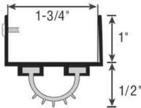
779S Door Shoe Mill/Vinyl
