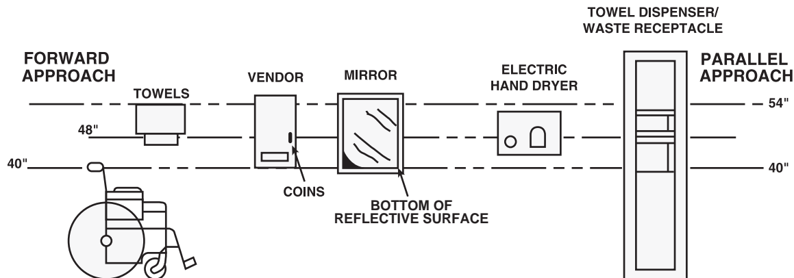
Diagram above shows ADA recommended mounting heights for washroom accessories. A minimum of 30" by 48" clear floor space is required in front of all accessible fixtures and accessories.
