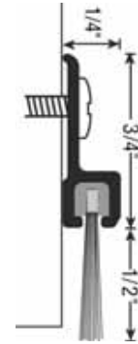
802S Astragal and/or Frame Seal
