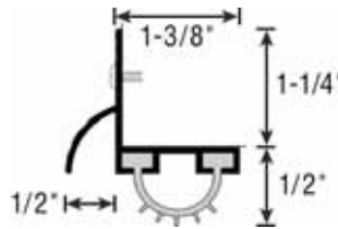
777S Door Shoe Mill/Vinyl
