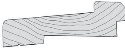
Standard "Set-Up" Sapele Mahogany** Sill Inswing Solid
