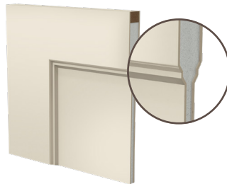
Stepped Sticking
