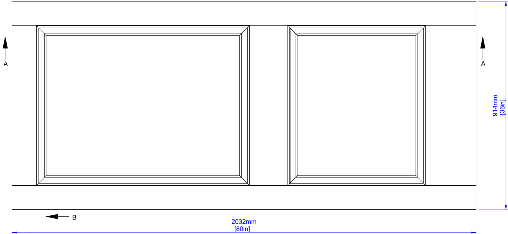
TWO PANEL 35 mm (1 3/8") Two Panel 19 mm Raised SGL-2S Standard VG Ovolo Sticking
