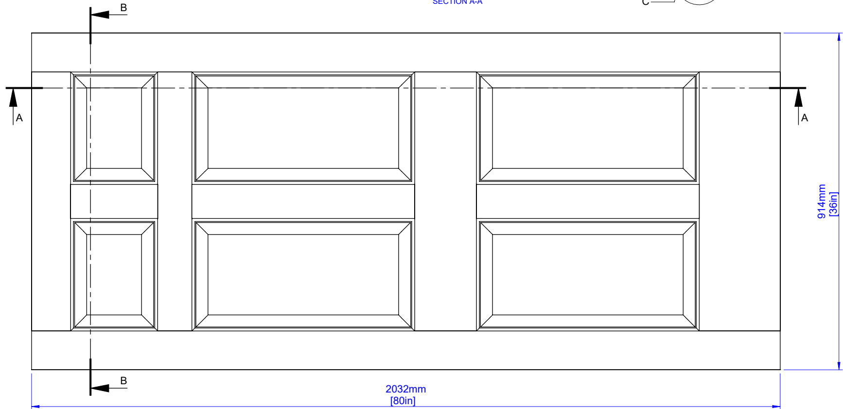
COLONIAL 35 mm (1 3/8") Six Panel 19 mm Raised SGL-2S Standard VG Ovolo Sticking
